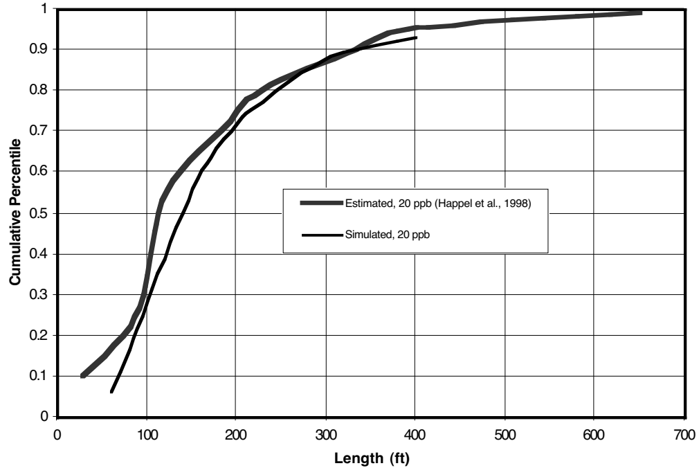
Figure 10. Estimated (Happel et al., 1998) and simulated MTBE plume lengths, circa 1995-96.
