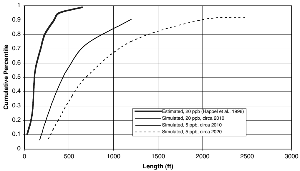
Figure 11. Simulated future MTBE plume lengths, circa 2010 and 2020.
