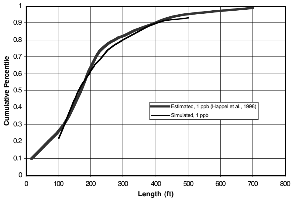
Figure 9. Estimated (Happel et al., 1998) and simulated benzene plume lengths, circa 1995-96.
